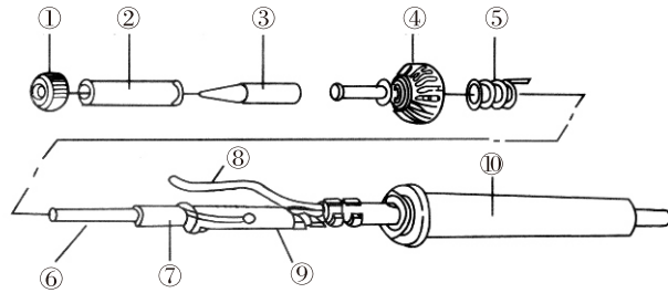
AT938D diagram (7)
